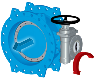
Design 01: • Standard • Gear left side • opening with flow direction
