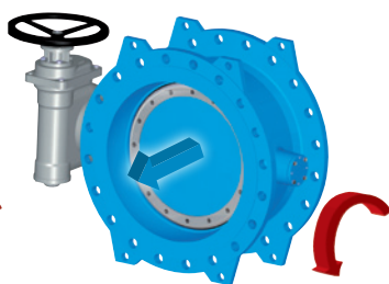
Design 02: • Optional • Gear right side • opening with flow direction
