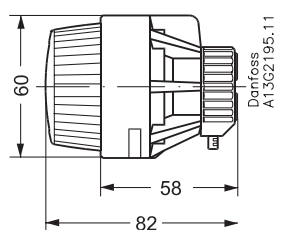
Tamperproof model RA 2920
