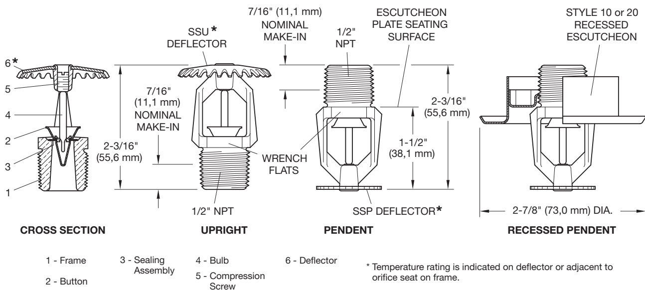
FIGURE 2 QUICK RESPONSE SERIES TY-FRB UPRIGHT (TY2131) AND PENDENT (TY2231) SPRINKLERS 4.2 K-FACTOR, 1/2 INCH NPT
