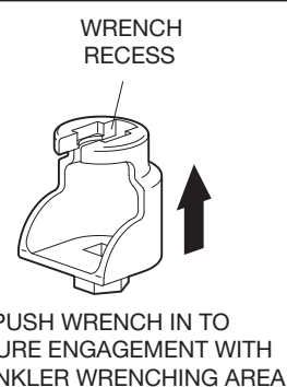
FIGURE 15 W-TYPE 7 RECESSED SPRINKLER WRENCH
