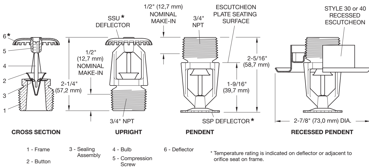
FIGURE 4 QUICK RESPONSE SERIES TY-FRB UPRIGHT (TY4131) AND PENDENT (TY4231) SPRINKLERS 8.0 K-FACTOR, 3/4 INCH NPT
