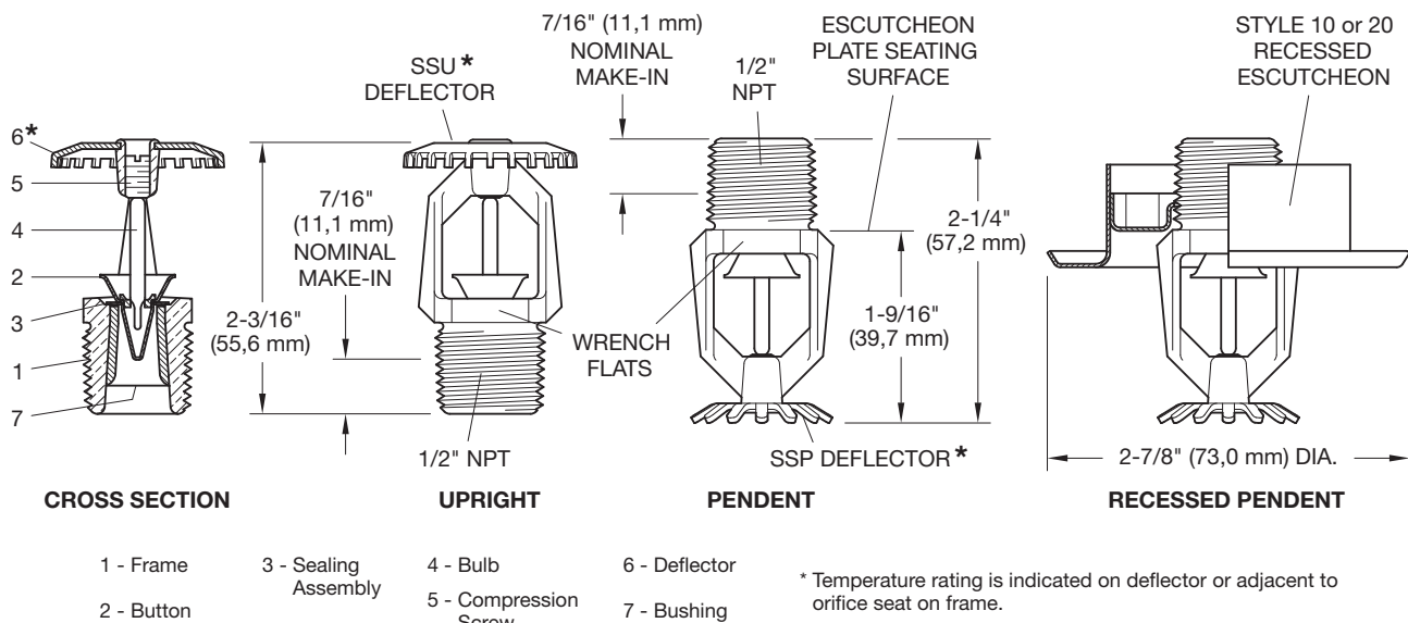
FIGURE 1 QUICK RESPONSE SERIES TY-FRB UPRIGHT (TY1131) AND PENDENT (TY1231) SPRINKLERS 2.8 K-FACTOR, 1/2 INCH NPT
