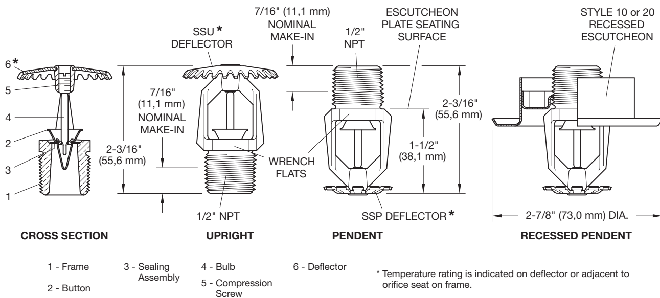
FIGURE 3 QUICK RESPONSE SERIES TY-FRB UPRIGHT (TY3131) AND PENDENT (TY3231) SPRINKLERS 5.6 K-FACTOR, 1/2 INCH NPT
