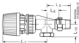
UK-angle valve body with thermostatic sensor RA 2990
