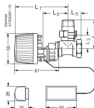
Angle valve body with thermostatic sensor RA2992
